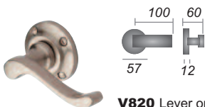
V820 Lever on Rose in all finishes shown
