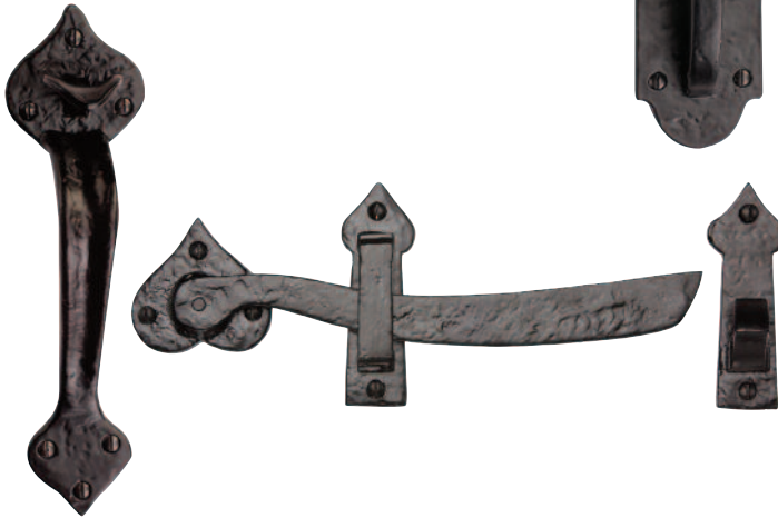
TC567 Handle height: 212mm Gate Latch length: 238mm
