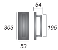
V1155 Pull Handle on Plate
