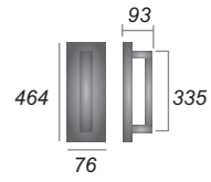
V1162 Pull Handle on Plate
