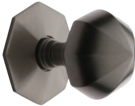
V880 Faceted Centre Door Knob Base 66mm Knob 57mm Projection 81mm
