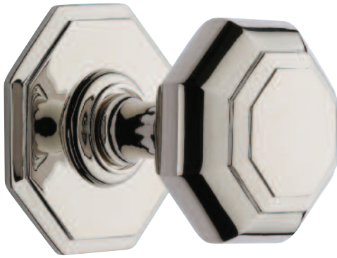
V890 Centre Door Knob Base 82mm Knob 71mm Projection 83mm
