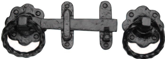
TC543 Ring Handle diameter: 72mm Ring base diameter: 72mm Gate Latch length: 170mm
