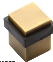
V1089 Floor Mounted Door Stop 30mm Square (including buffer) Height: 35mm
